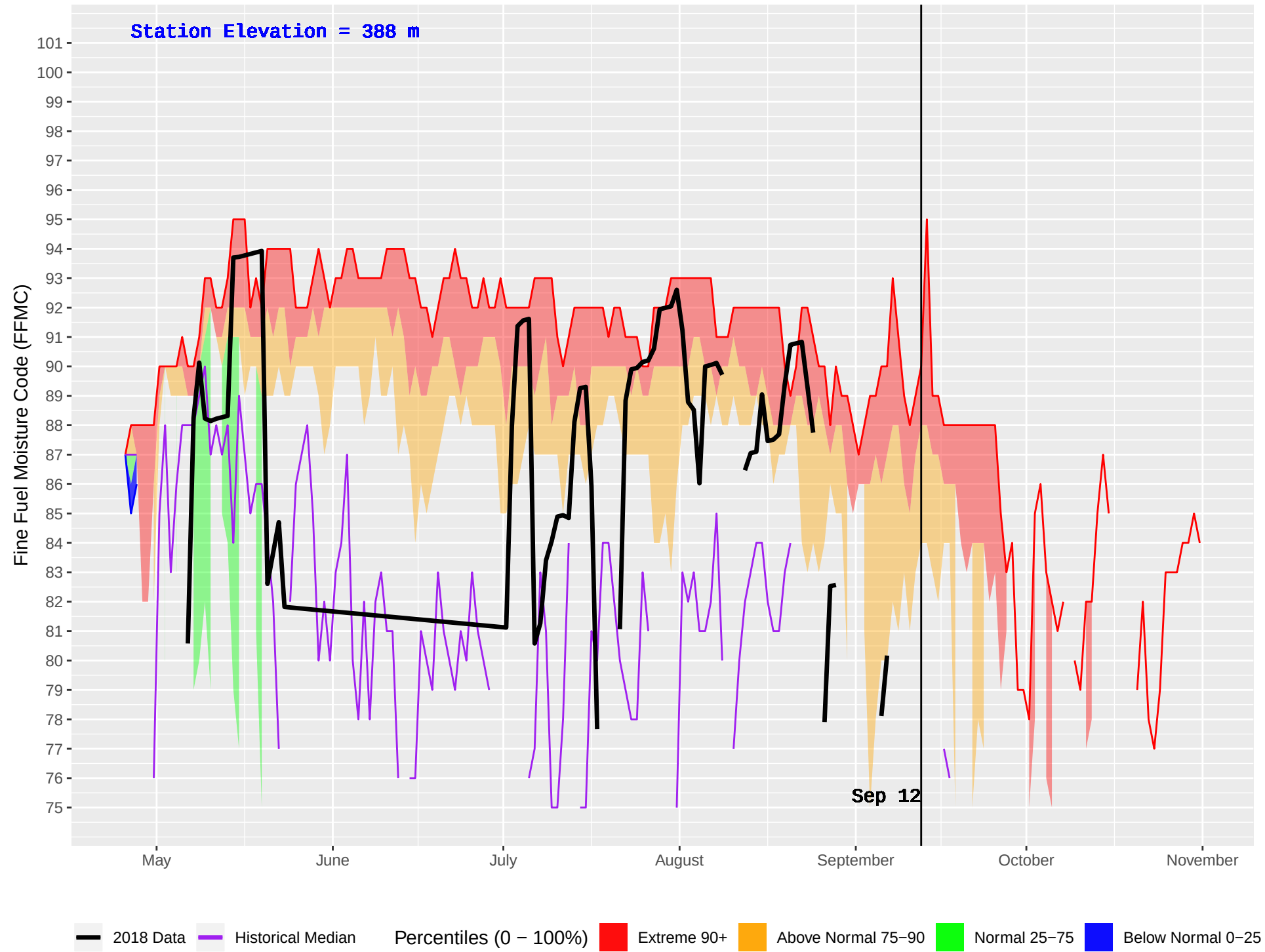
BELL-IRVING (432) : Historical (1986–2016) and Current (2018) Daily Fine Fuel Moisture Code (FFMC)
