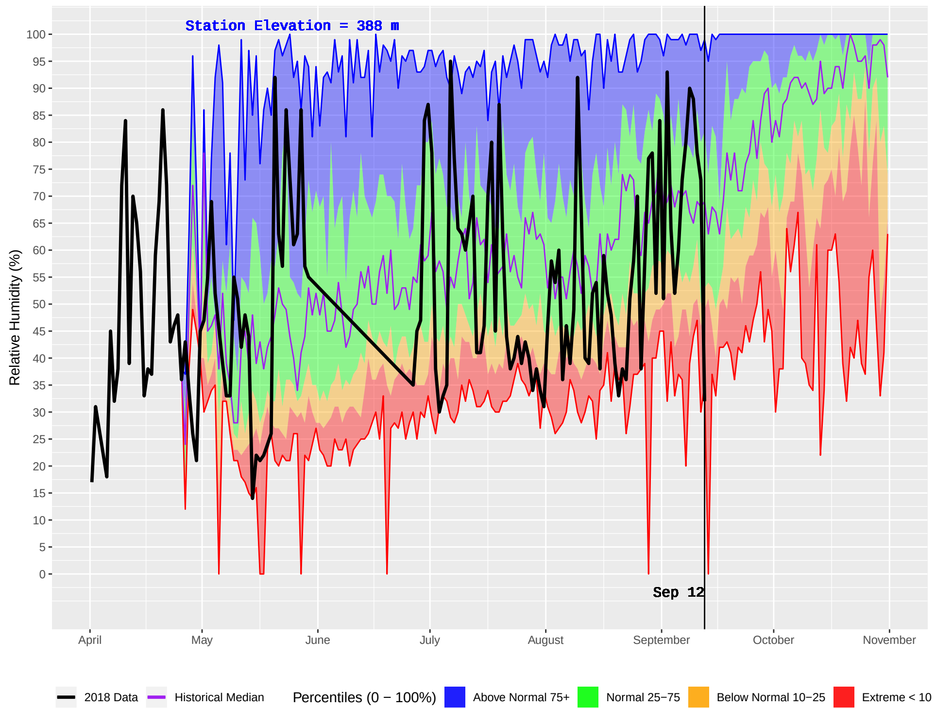
BELL-IRVING (432) : Historical (1986–2016) and Current (2018) Daily Relative Humidity
