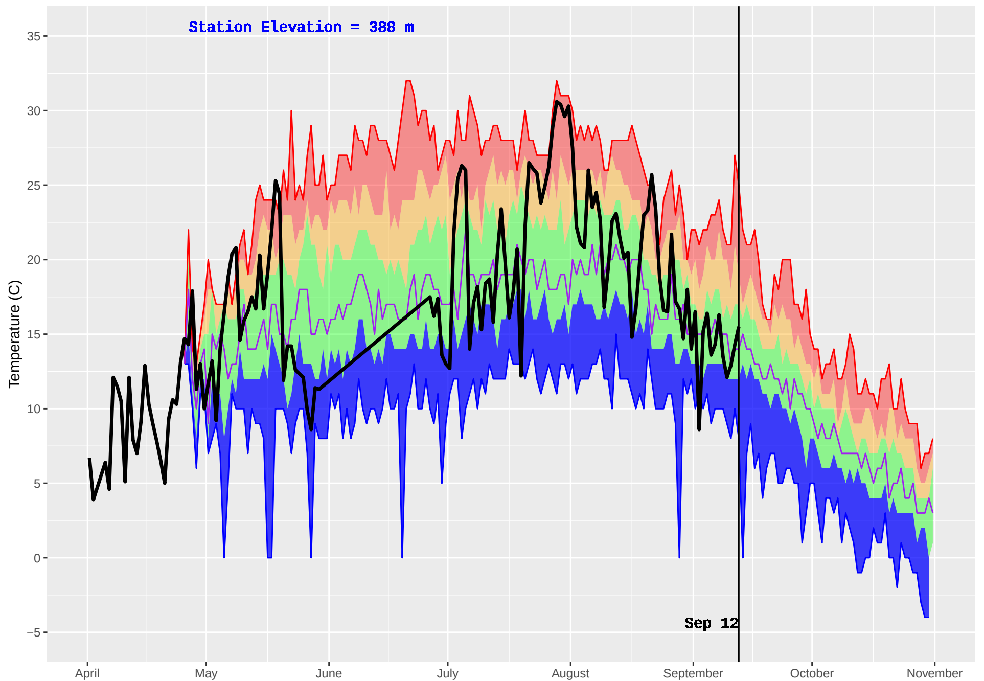
BELL-IRVING (432) : Historical (1986–2016) and Current (2018) Daily Temperature
