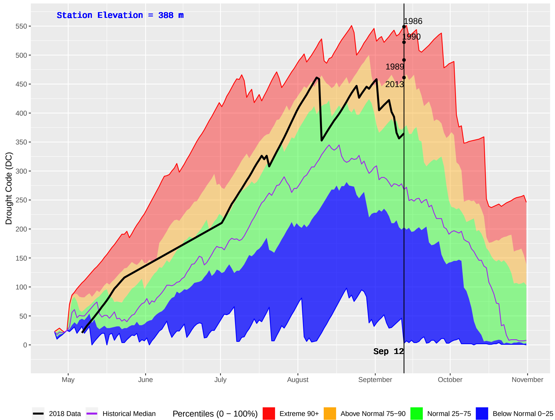
BELL-IRVING (432) : Historical (1986–2016) and Current (2018) Daily Drought Code (DC)
